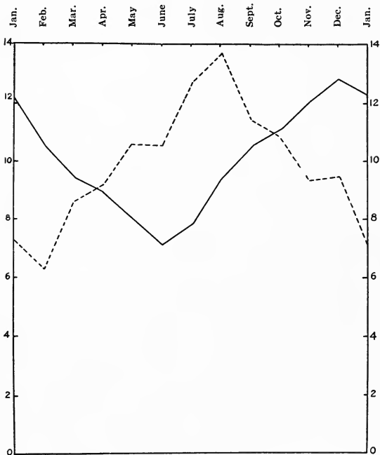
Fig. 12. Seasonal distribution of earthquakes.
